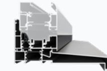
Folding and Sliding Door 190mm cill
