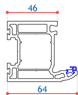
105033 64mm Lower Sash Steel Box 113314 Aluminium Box 115275
