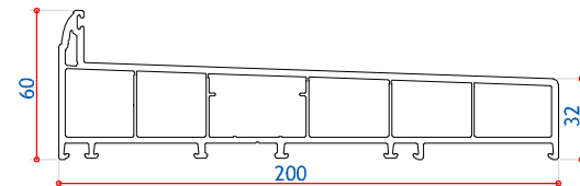
105410 200mm Cill Section Steel Box 113073
