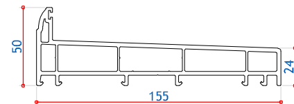
105037 155mm Cill Section Steel U Channel 113321
