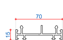
114039 15mm Frame Ext
