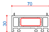
114014 30mm Frame Ext 38 x 15mm Steel Box 113073
