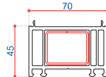
114202 45mm Frame Ext 38 x 30mm Steel Box 113271
