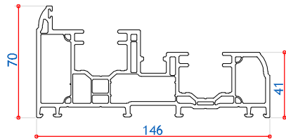
105411 70mm Outer Frame Steel Box 113073
