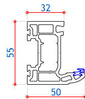
105032 50mm Upper Sash Steel Box 113020 Aluminium Box 115010
