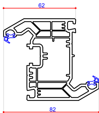
103364 82mm Tilt N Turn Sash/Z Mullion Steel U Channel 113413 Steel P Section 113417
